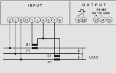
Three-phase 3Ph network, unbalanced load (aron L1-L3)
