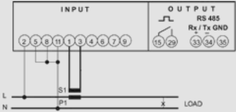
Single-phase network,
